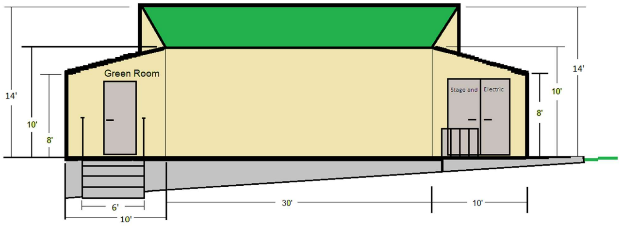
Rear View
